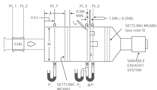
Figure 12 Outlet Chamber ANSI/AMCA STANDARD 210-85
